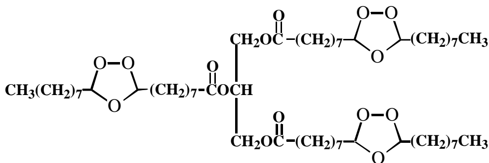
Figure 3 The structure of triolein triozonide
